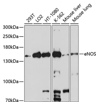
Fig. 1. Western blot analysis of extracts of various cell lines, using eNOS antibody at 1:1000 dilution. Secondary antibody: HRP-labeled Goat Anti-Rabbit IgG(H+L) (A0208) at 1:1000 dilution. Lysates/proteins: 25µg per lane. Blocking buffer: QuickBlock™ Blocking Buffer (P0231). Detection: BeyoECL Star (P0018A). Exposure time: 1s.
